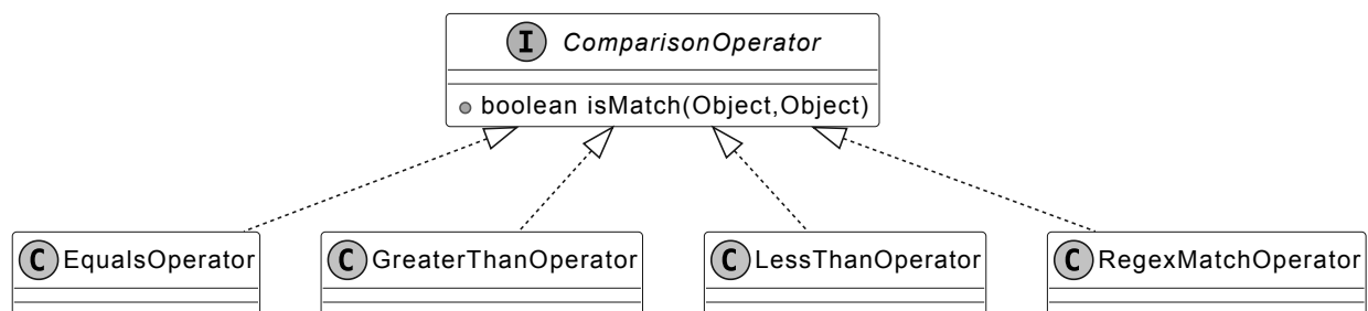
ComparisonOperator interface and concrete classes
