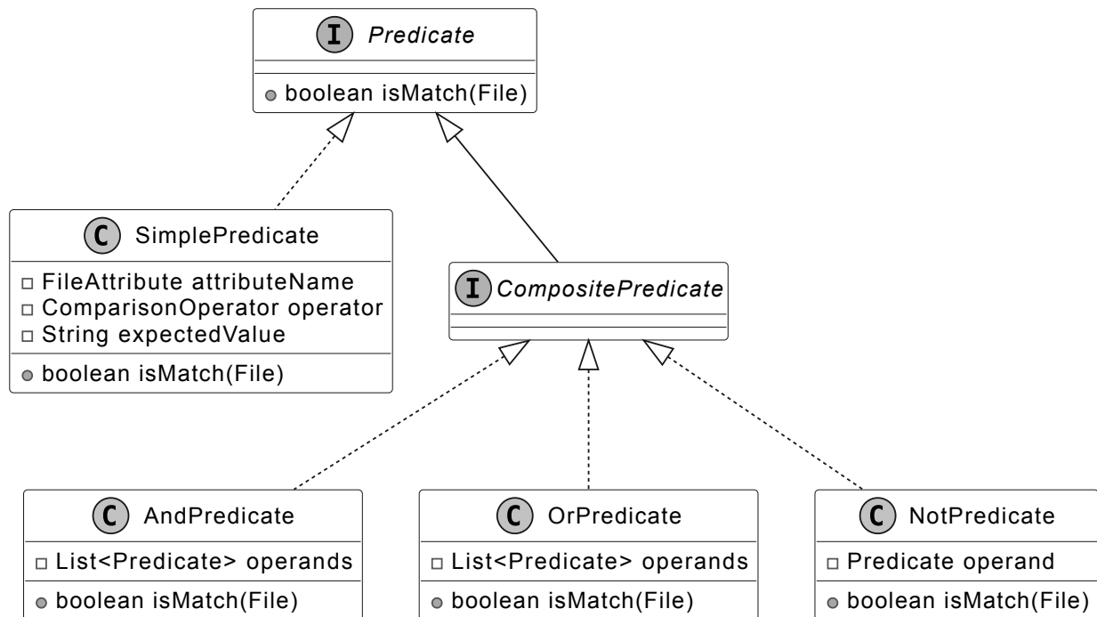
CompositePredicate interface and concrete classes
