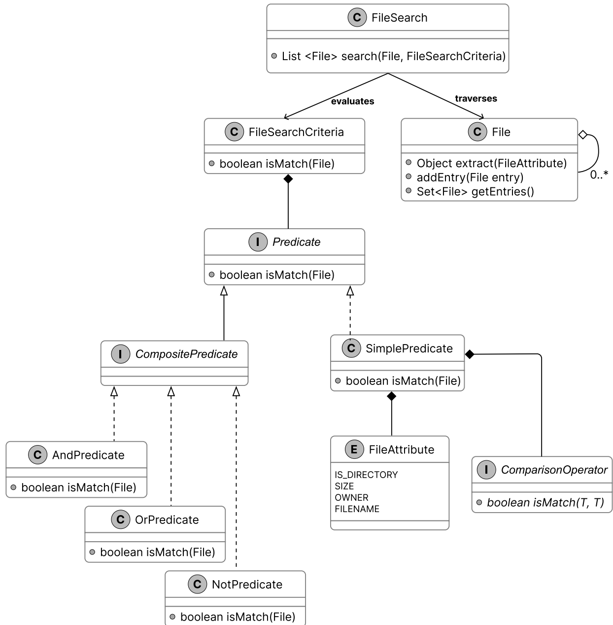
Class Diagram of File Search
